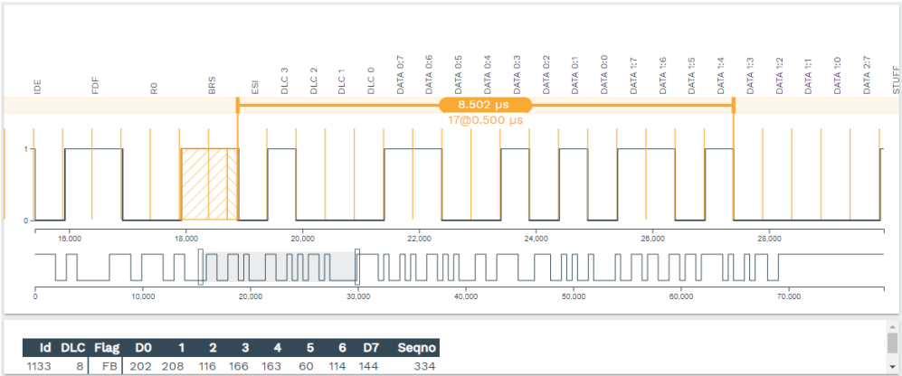
Figure 8: Using information from Kvaser CANtegrity, the time between two edges can be measured.
