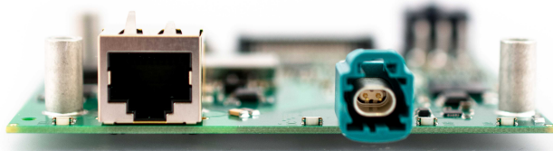
Figure 2: Ethernet connectors on Kvaser Arcus 100/1000BASE-T1 H-MTD
