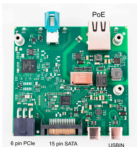
Figure 4: Connectors that supply the Kvaser Arcus 100/1000BASE-T1 H-MTD
