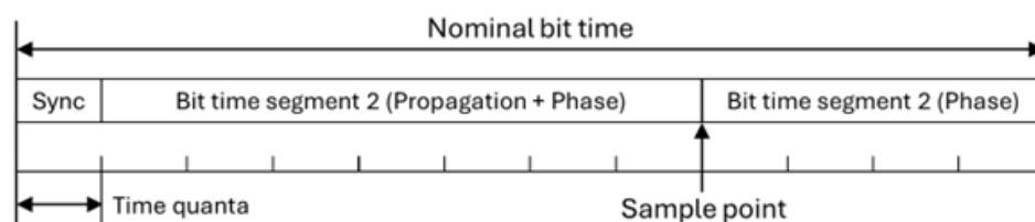
Figure 2: Bit timing.
