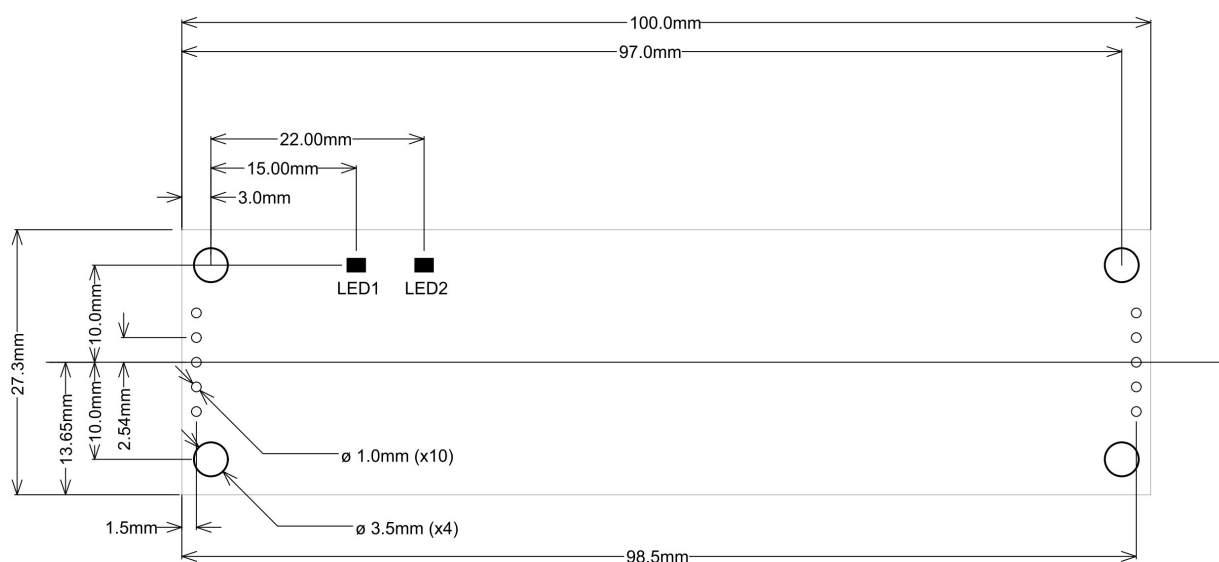
Figure 4: LEDs and mounting holes on the Kvaser Leaf v3 CB.
