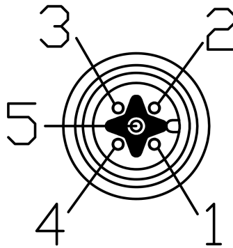
Figure 5: 5-pole male M12 Connector
