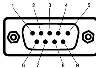
Figure 4: The D-SUB 9 connector pin numbers
